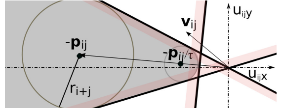
(b) Constraint (grey) of relative reference velocities (\mathbf{u}_i - \mathbf{u}_j) leading to a future collision.
