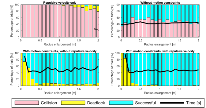
Fig. 14. Performance comparison for four instances of the method in the antipodal exchange scenario of Fig.12 with ten simulated robots. We display the percentage of trials that ended in collision, deadlock or succeeded, over one hundred simulations for each radius enlargement \epsilon . Top left: the preferred velocity corrected with the repulsive velocity is applied directly to the robots. Top right: the optimization method without motion constraints (ORCA). Bottom left: The method with motion constraints ( \epsilon CCA), but without correcting the preferred velocity with the repulsive velocity. Bottom right: The method with motion constraints and repulsive velocity ( \epsilon CCA). The same parameters are used in all simulations.
