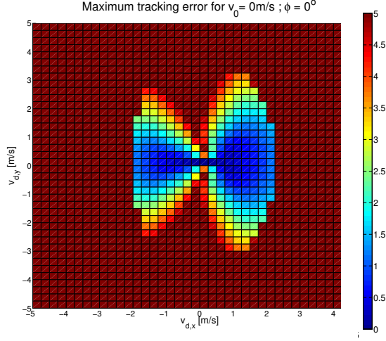
Fig. 4. Maximum tracking errors in [m], and saturated at 5 m, for a car-like robot [29] and for varying values of the control velocity \mathbf{u} . In this example the initial velocity is set to \mathbf{v}_i^0 = 0\text{m/s} and the initial steering angle to \phi = 0^\circ . As expected, the robot can easily track control velocities aligned with its orientation, but experiences high tracking errors for control velocities in the perpendicular direction (which would require the car to rotate).
