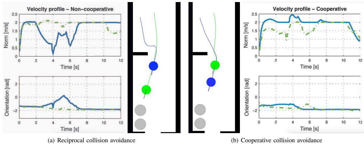
Fig. 17. Comparison of the \epsilon CCA reciprocal and cooperative approaches for computing the pair-wise distributed avoidance constraints. Two robots (blue/green circles) navigate in a corridor (white = free space) towards their goals (grey circles). In the middle, path of the robots. In the sides, velocity profile and orientation over time for both robots during the interaction (dashed green and solid blue).
