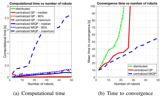
Fig. 16. Antipodal position exchange in a circle, for varying number of robots with bicycle kinematics. Comparison of distributed \epsilon CCA (light green), centralized convex QP \epsilon CCA (dark red) and centralized non-convex MIQP \epsilon CCA (dark blue). a) Computational time of the approach, where the green line is below the red line. b) Mean time to convergence to the antipodal positions in the circle.
