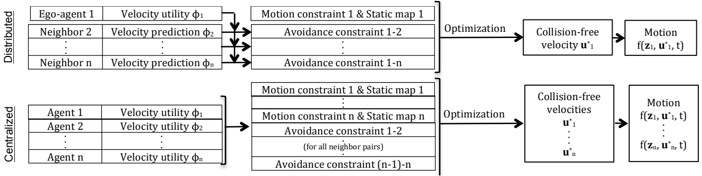
Fig. 2. Local motion planning. Overview of the approaches for distributed and centralized collision avoidance.
