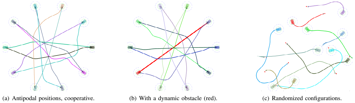
Fig. 12. Trajectories of ten car-like robots moving from their initial to a goal (red circles) configuration.
