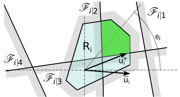
Fig. 8. Optimization in velocity space for a unicycle robot i with current orientation \theta_i in a scenario with five robots. The optimal collision-free velocity \mathbf{u}_i^* satisfies the linear constraints (marked with a straight line with the gray side indicating the infeasible half-plane) and minimizes the distance to the preferred velocity \bar{\mathbf{u}}_i . The feasible region is highlighted in green.
