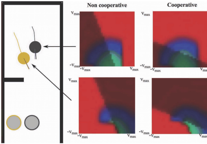
Fig. 6. Example of velocity utility for two robots (black/brown) navigating towards their goal (grey disk) in a corridor environment, and their reciprocal/cooperative partition for distributed collision avoidance (shadowed area represents the unfeasible side of the constraint). The maximum of the velocity utility is displayed in light blue, decreasing towards dark blue and with its minimum (zero value) red. Values are scaled and independent in both images. For visualization, the axis are aligned with the map.
