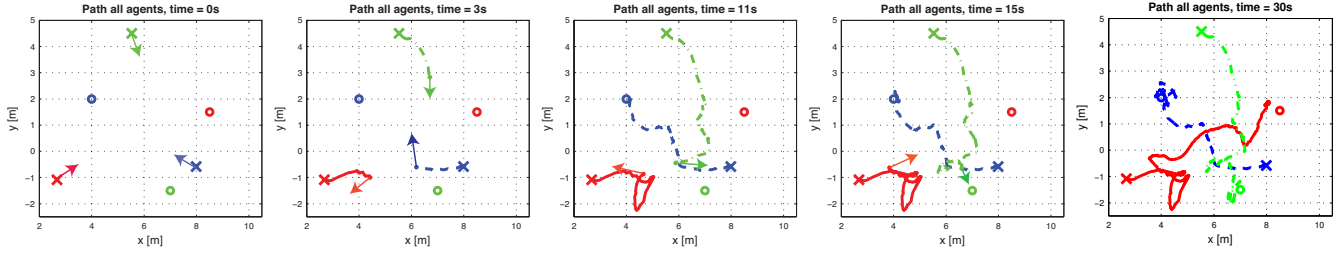
(b) Collision avoidance with repulsive velocities. The paths of the boats are displayed at representative intervals. Total time is 30 seconds
