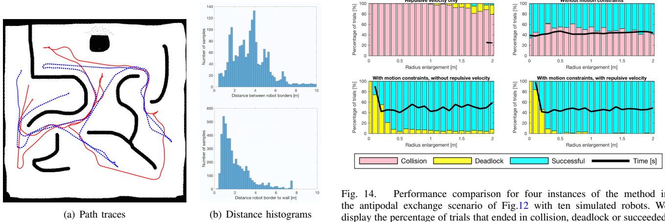
Fig. 13. Two simulated wheelchairs navigate, at a preferred speed of 5m/s, between several goal positions in a complex environment and successfully avoid collisions via cooperative \epsilon CCA. (a) Traces of the path of both robots and obstacle map. (b) Histograms of border to border inter-robot distance (top) and robot border to wall (below). No collisions are observed.
