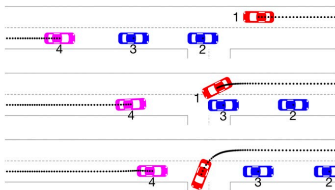
Fig. 4. Unprotected left turn of an AV (red; i=1 ) with oncoming traffic. As the AV approaches the intersection, two egoistic cars (blue; i=2, 3 ) continue and do not yield. A third altruistic car (magenta; i=4 ) yields by slowing down, allowing the AV to complete the turn in the gap.
