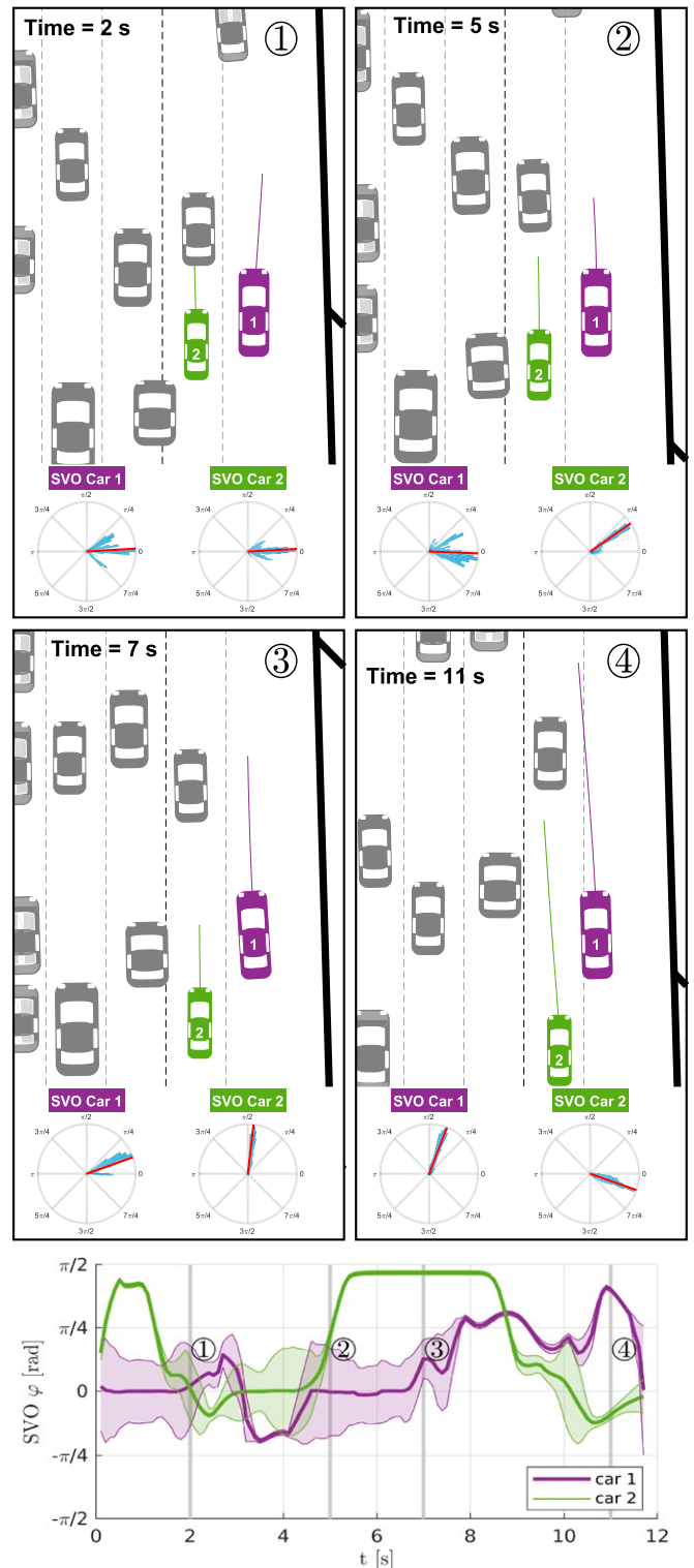
Fig. 2. (Upper) Snapshot of NGSIM dataset with n = 2 active cars (purple and green) and n = 50 obstacle cars (gray). Here, car 1 (purple) is attempting a merge and must interact with car 2 (green). The solid lines indicate the predicted trajectory from our algorithm. For SVO estimates at each frame, the blue represents the distribution, while the red line indicates our estimate. (Lower) The solid line indicates SVO estimate over time, with the shaded region representing the confidence bounds. Initially, car 2 does not cooperate with car 1 and does not allow it to merge. After a few seconds, car 2 becomes more prosocial, which corresponds to it “dropping back” and allowing the first car to merge.
